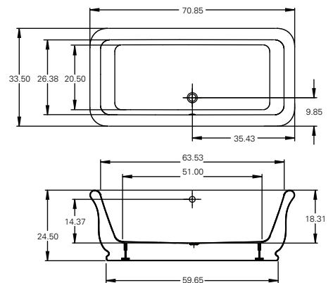
71FS33 Freestanding bathtub, 70 US Gal.
